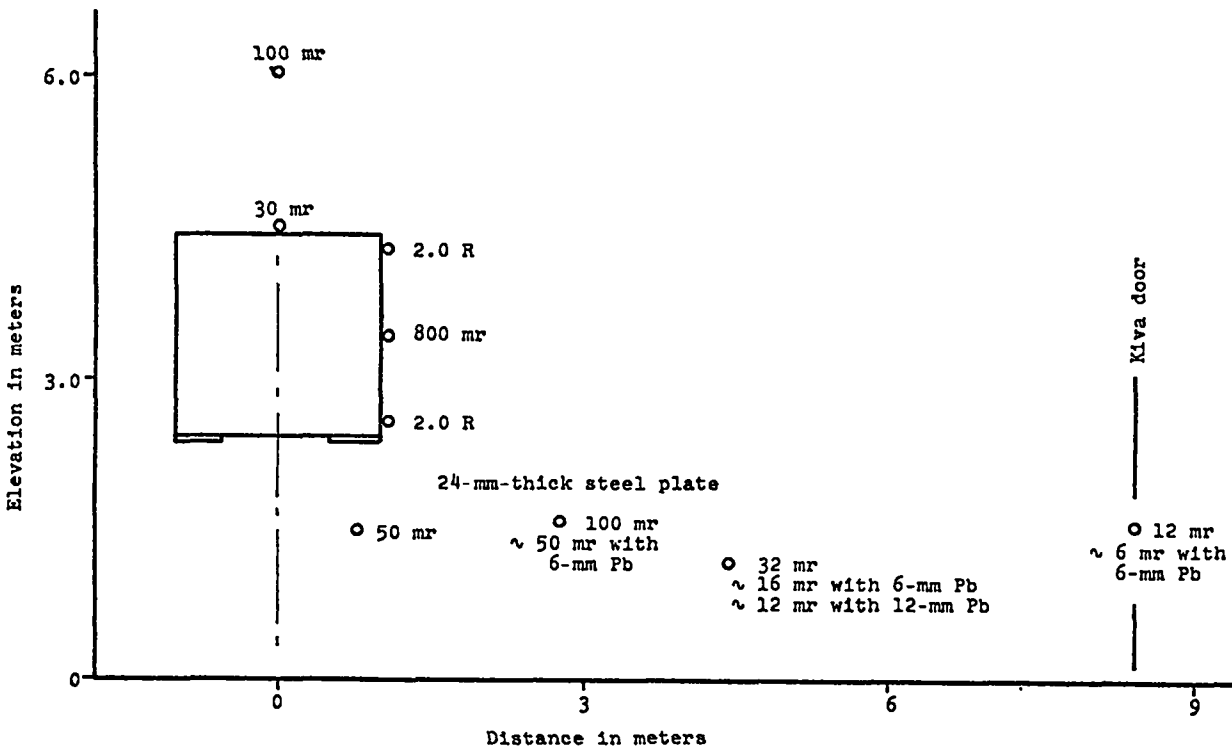
Fig. 6 Gamma radiation levels near PCA.
